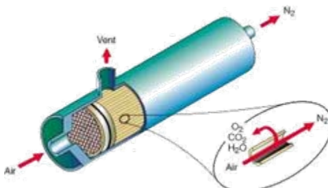
Membrane separator cross section
